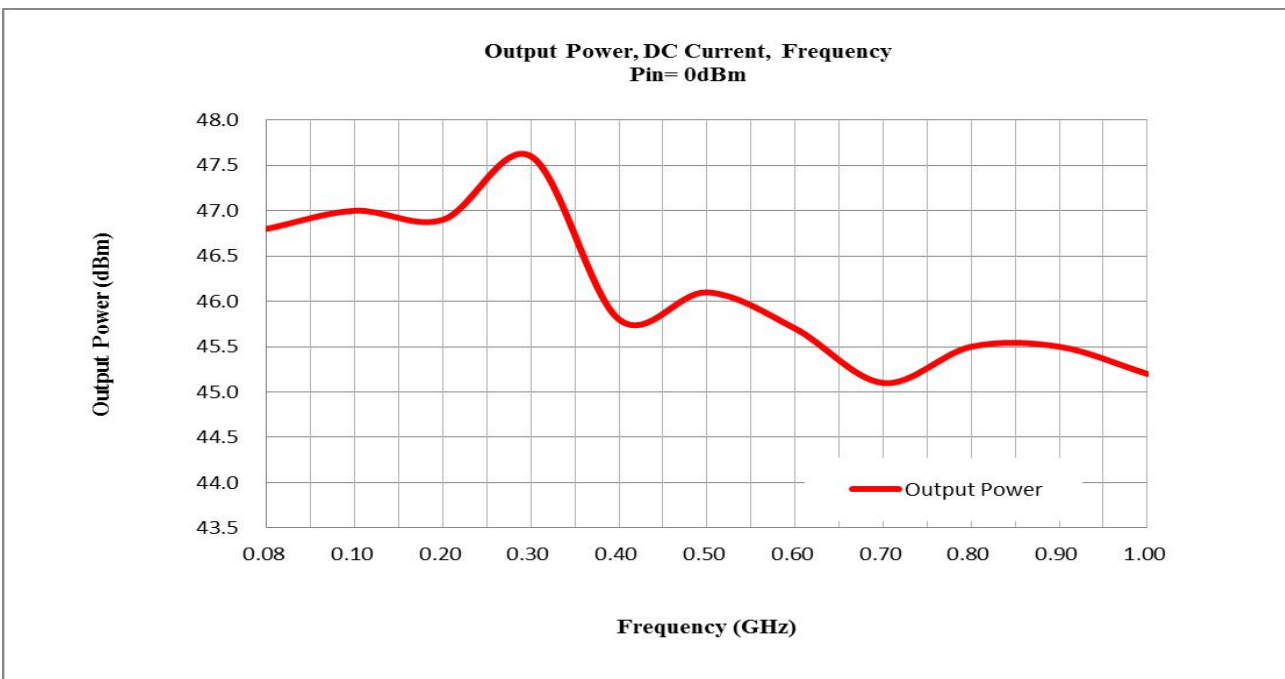
Graph 2: Output Power (High temp. +40±3°C)
