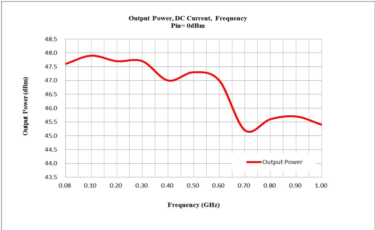
Graph 2: Output Power (High temp. +40±3°C)
